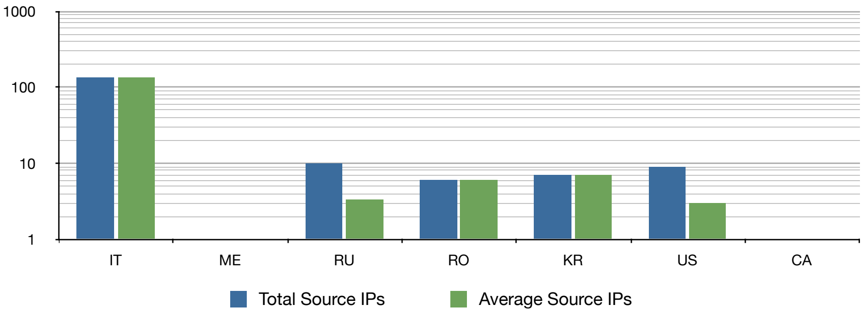
Interfree.it Botnet Events per Tier RFI
