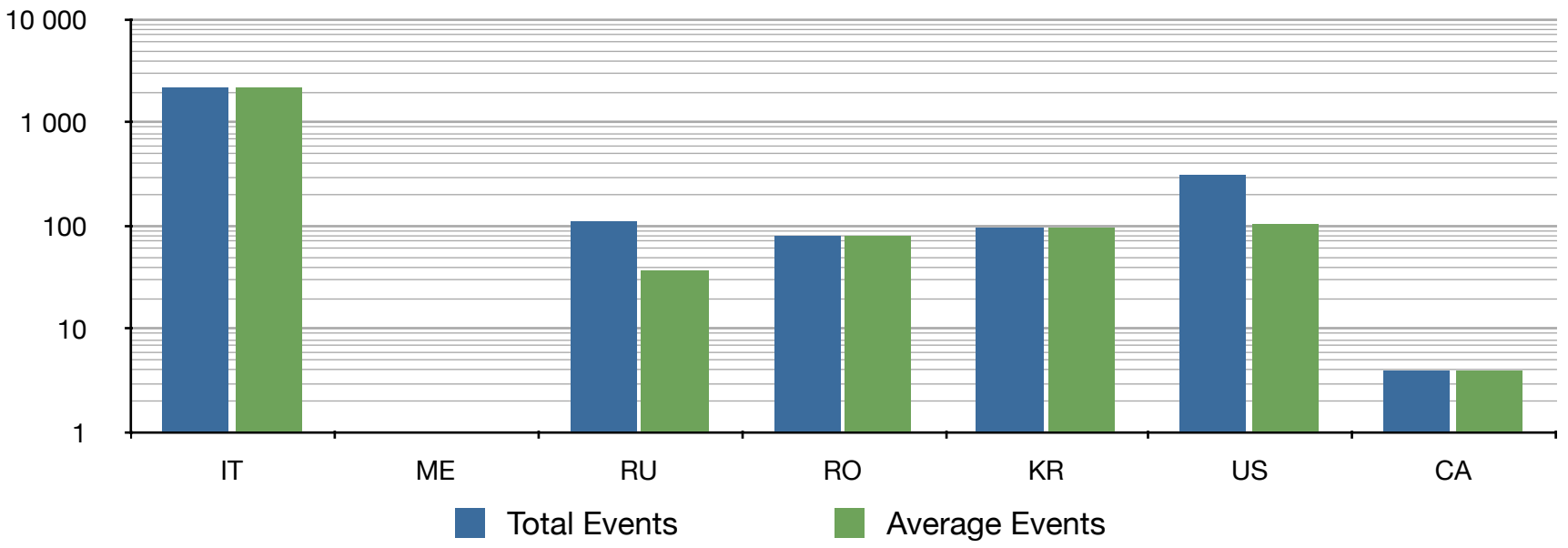
Interfree.it Botnet Total & Average Source IPs
