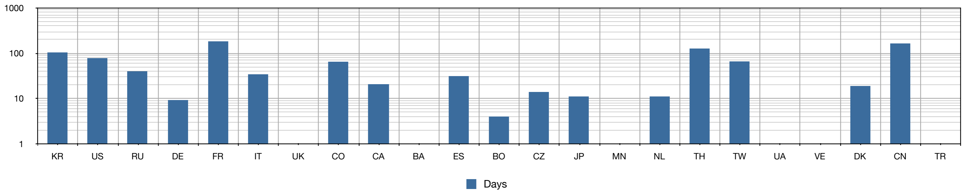
FileAve.com Botnet Average Lifetime
